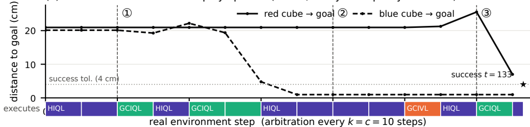
(a) WMPP on one cube-double-play episode (task 5; every fixed policy fails on it)
