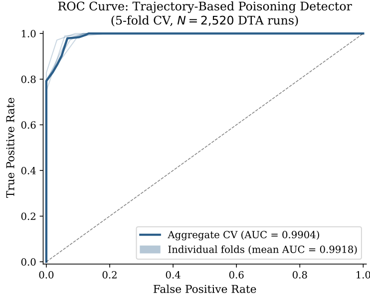
Figure 1: ROC curves for the Random Forest classifier. The aggregate curve (pooled out-of-fold predictions from 5-fold CV) achieves \text{AUC} = 0.9904 . Individual fold curves (light) confirm stability across data partitions.
