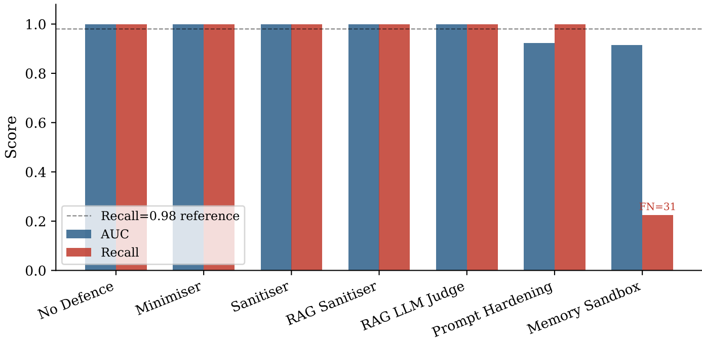
Detector Performance Across Defence Conditions
