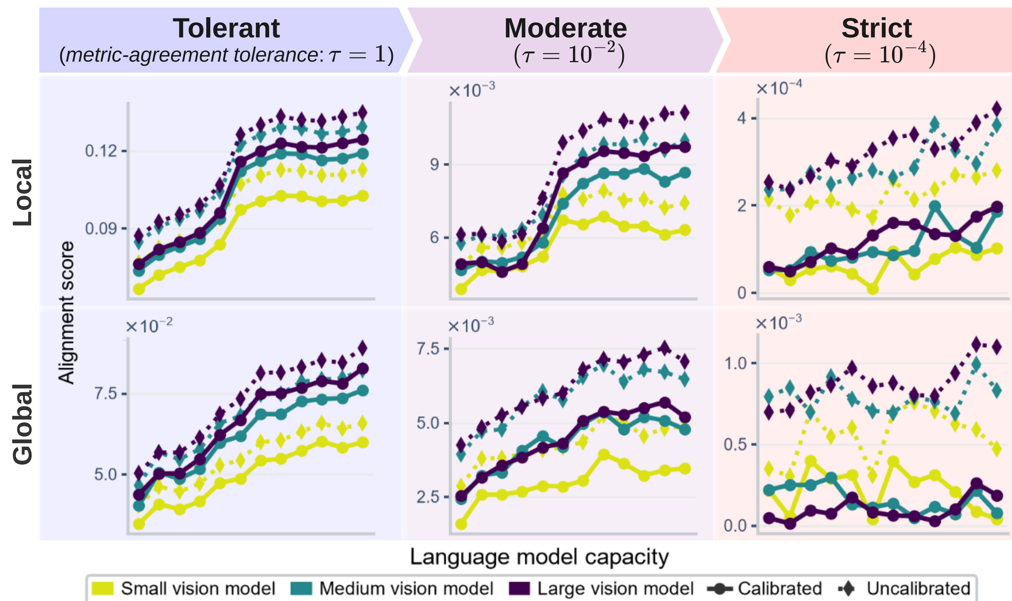
(b) Stricter metric agreement weakens convergence
