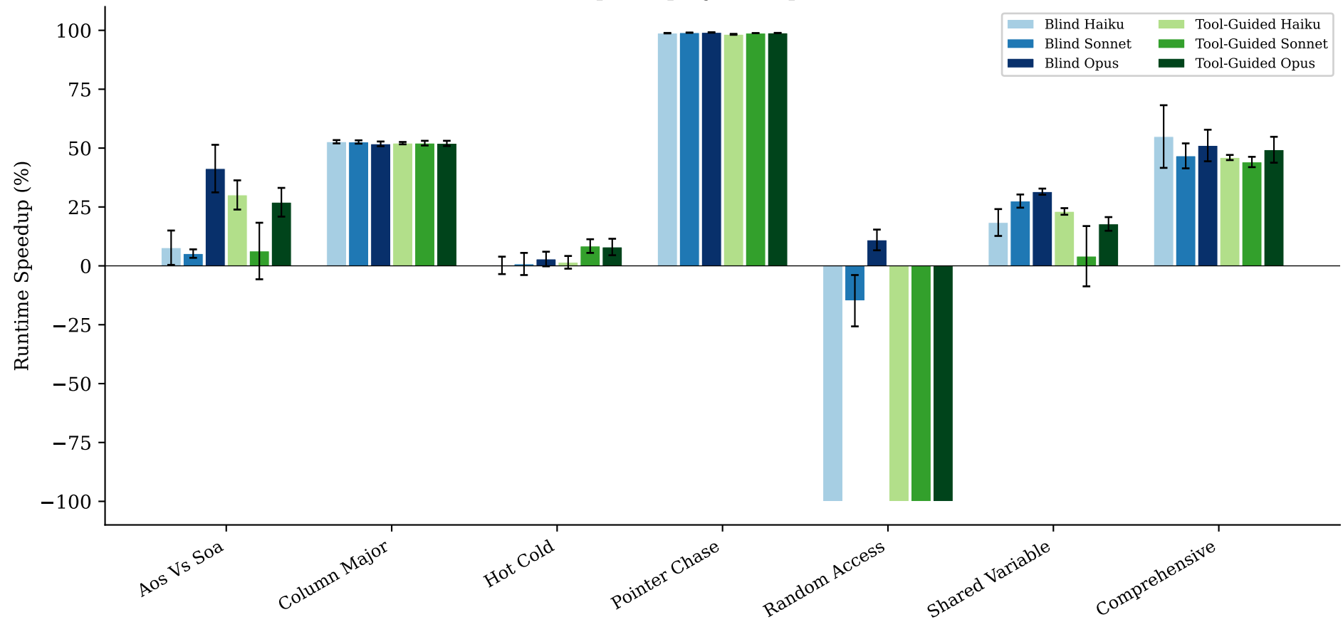
Runtime Speedup by Example and Method
