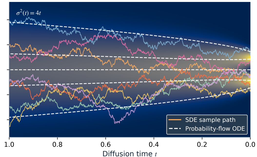
Reverse diffusion: noise to data
