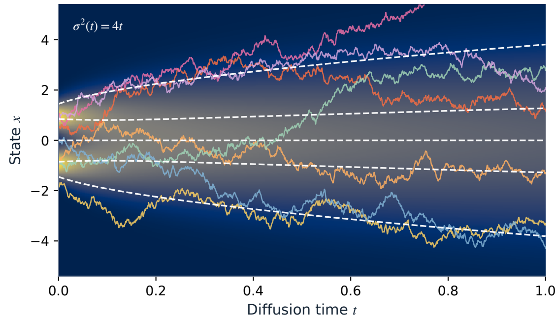
Forward diffusion: data to noise
