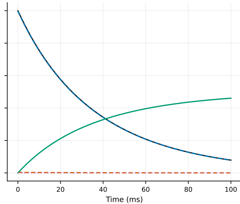
SOD-mediated
