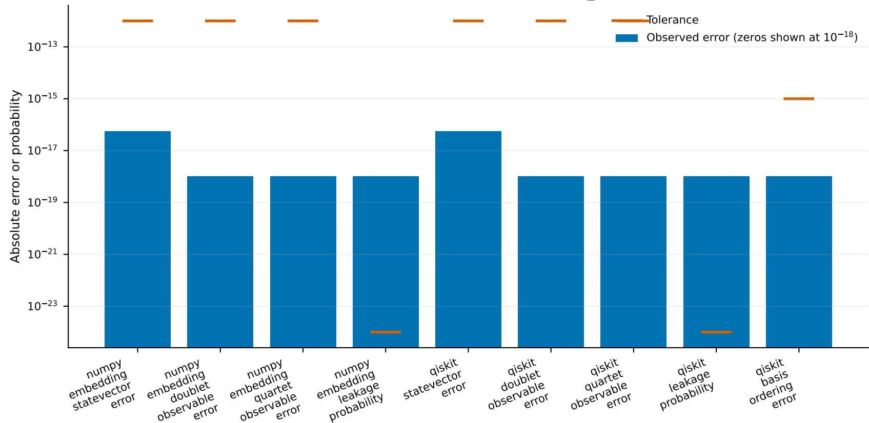
Three-qubit dense-unitary consistency: qiskit_executed
