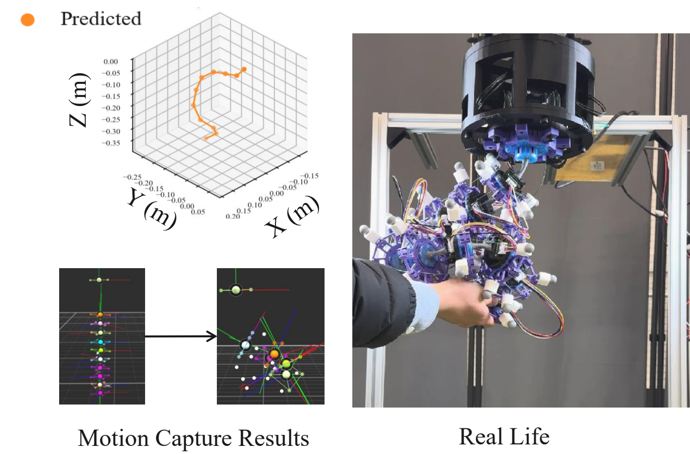
b) Pose estimation results of scenario 3 where the robot position is manipulated by hand. In this scenario the motion capture failed in tracking the reflective markers hence no ground truth is available, however our pose estimation still outputs a relatively accurate result under such large deformation.
