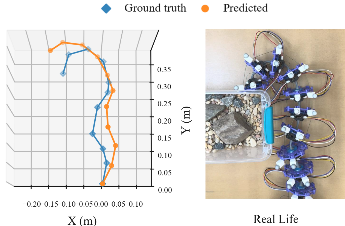
b) Pose estimation results of scenario 2 where the robot movement is blocked by a box of rocks. The computed RMSE of the prediction to ground truth is 0.0395 m
