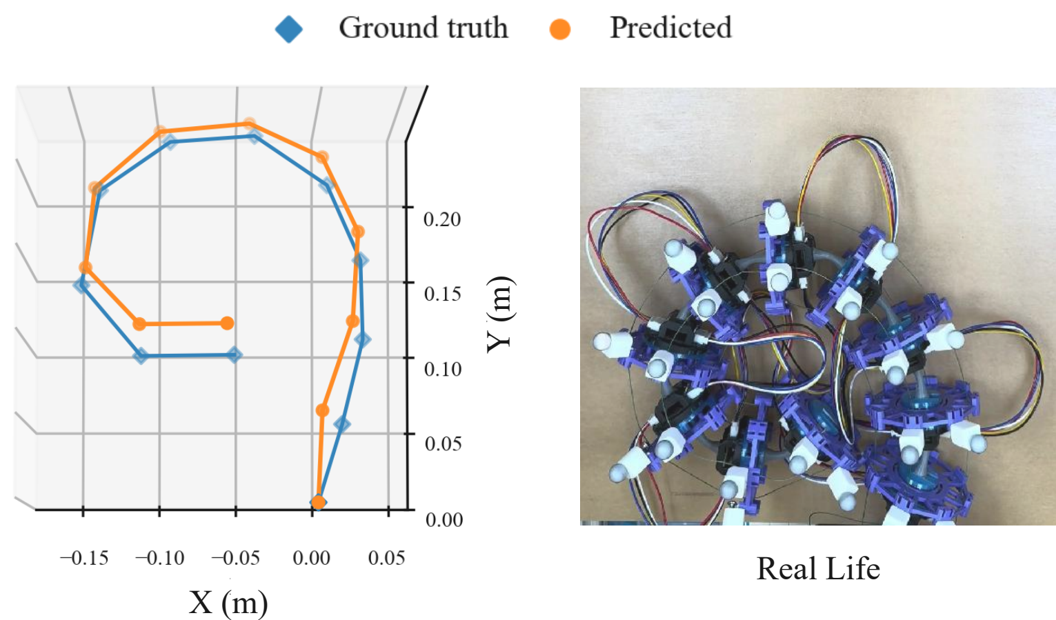
a) Pose estimation results of scenario 1 where the robot is allowed for free movements without restriction. The computed RMSE of the prediction to ground truth is 0.025483 m
