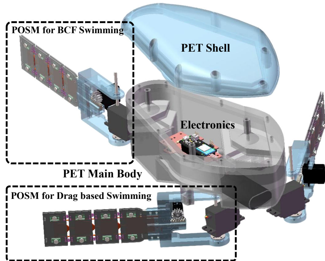
(b) Exploded View of Modular Swimming Platform
