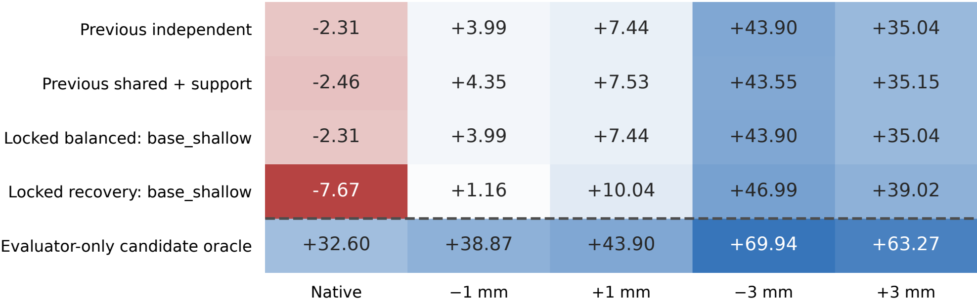
A MSE reduction versus KEEP (%) — positive is better
