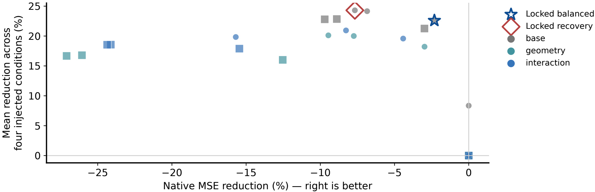
B All 24 locked working points — no replay-selected winner
