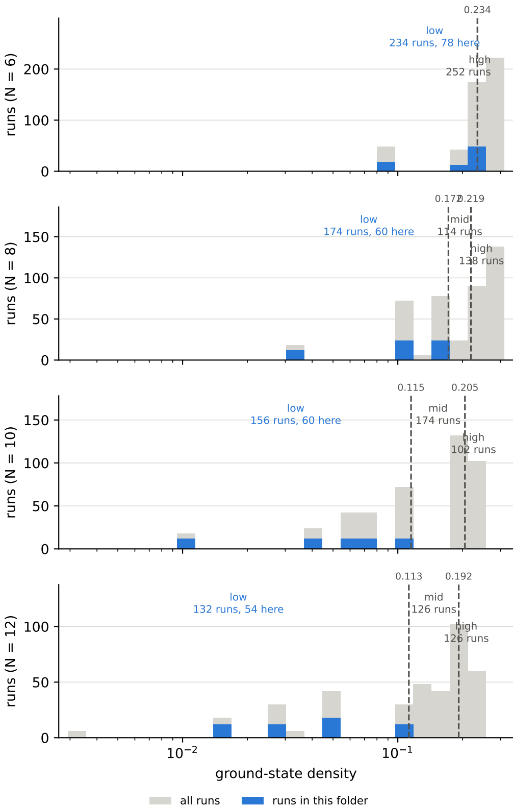
ground-state density over all runs, and the cuts behind the bins field B z = high, ground-state density = low
