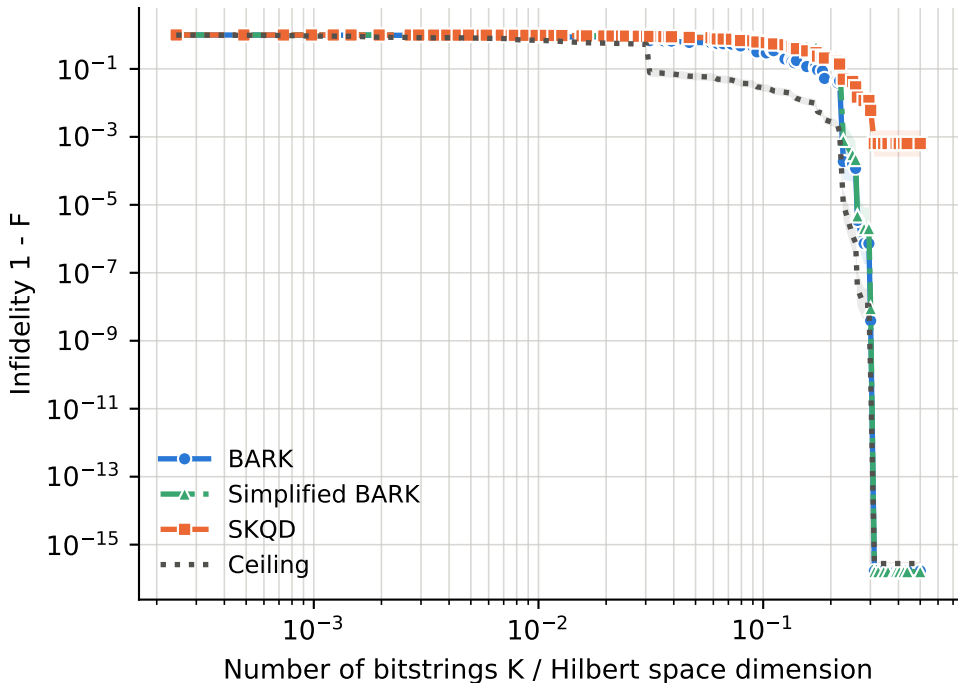
field B_z = low, ground-state density = high (band: standard error)
