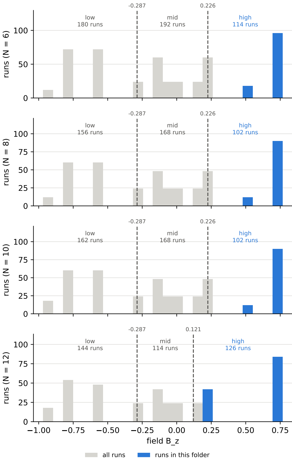
field B_z over all runs, and the cuts behind the bins field B_z = high, Hamiltonian density = all
