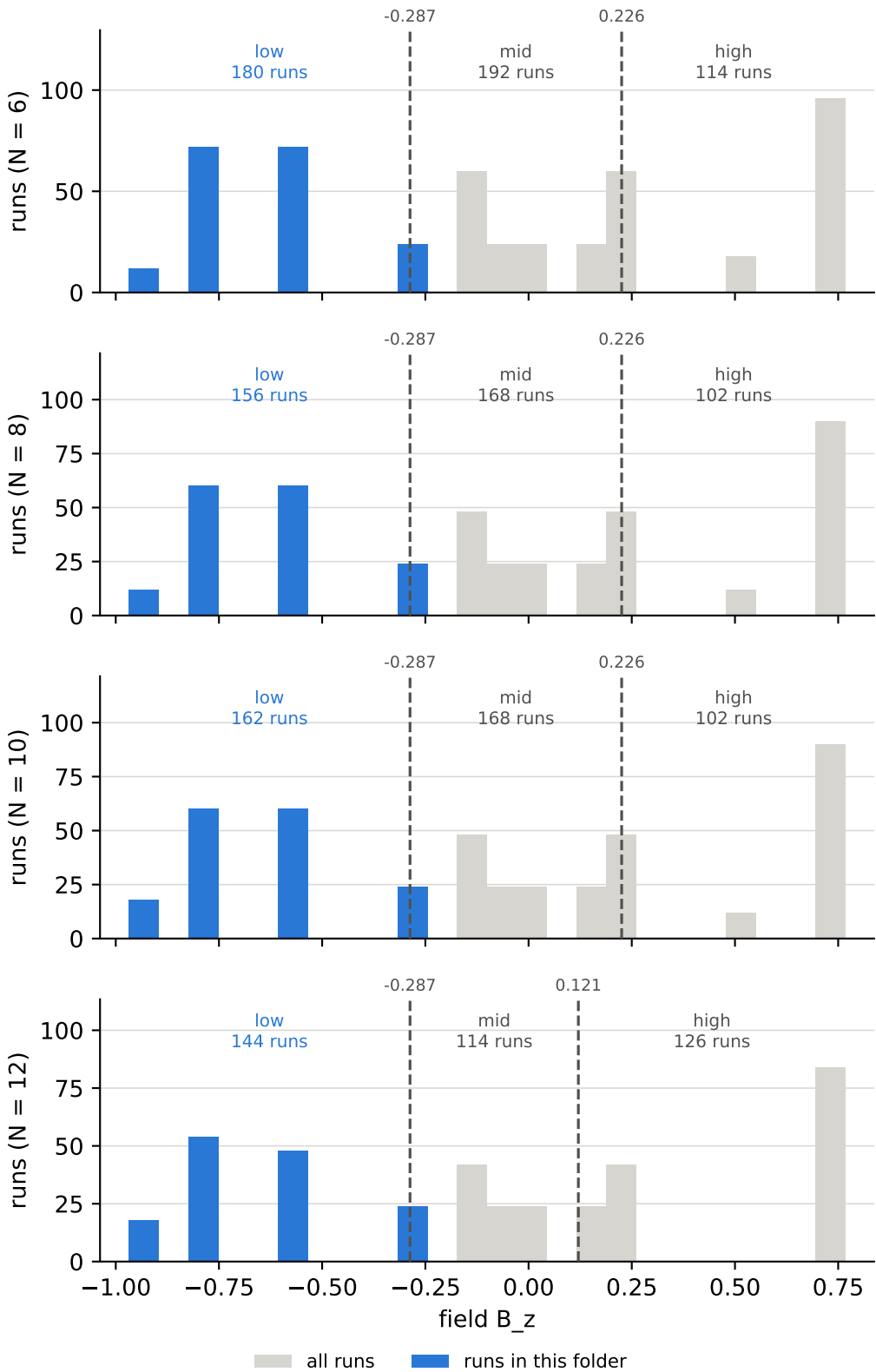
field B z over all runs, and the cuts behind the bins field B z = low, Hamiltonian density = all
