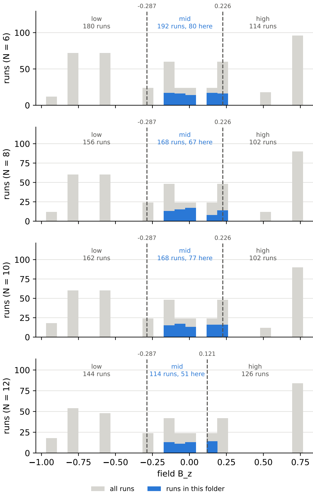
field B z over all runs, and the cuts behind the bins field B z = mid, initial overlap = mid
