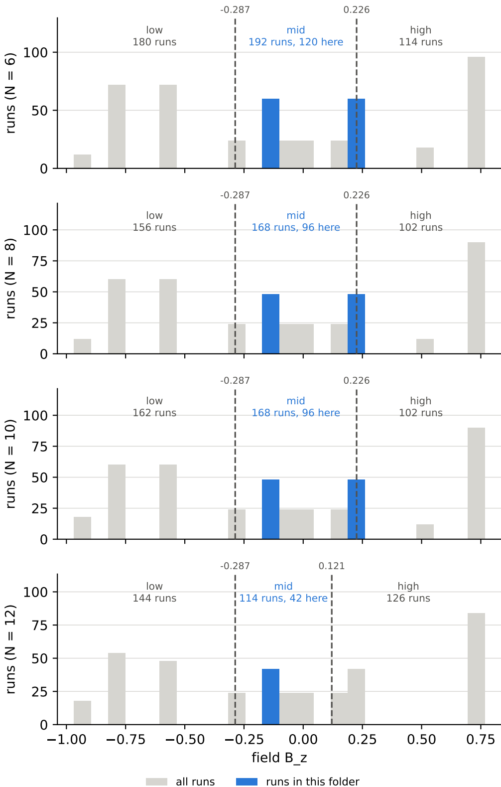
field B z over all runs, and the cuts behind the bins coupling J = mid, field B z = mid
