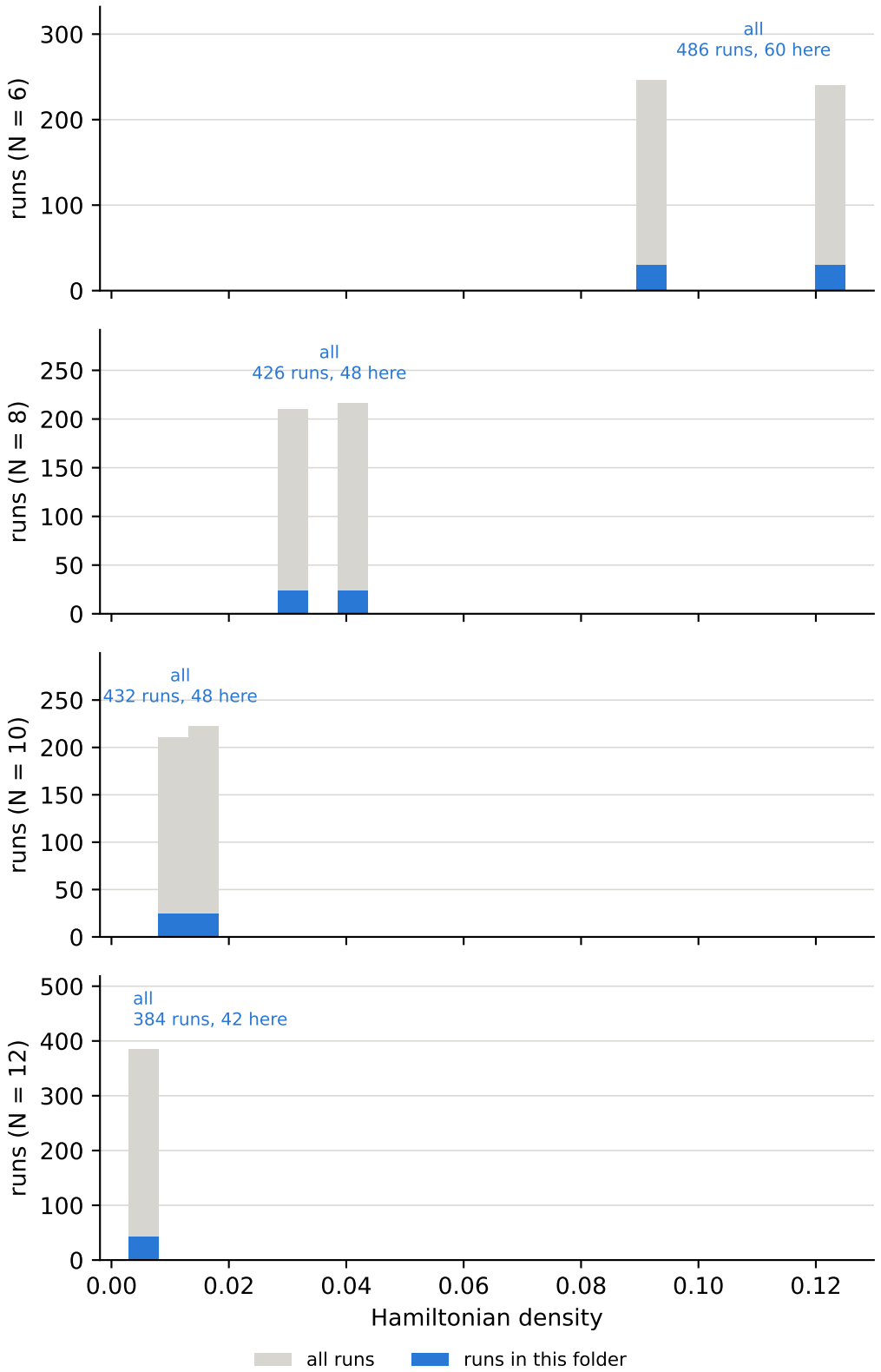
Hamiltonian density over all runs, and the cuts behind the bins coupling J = high, field B_z = high, Hamiltonian density = all
