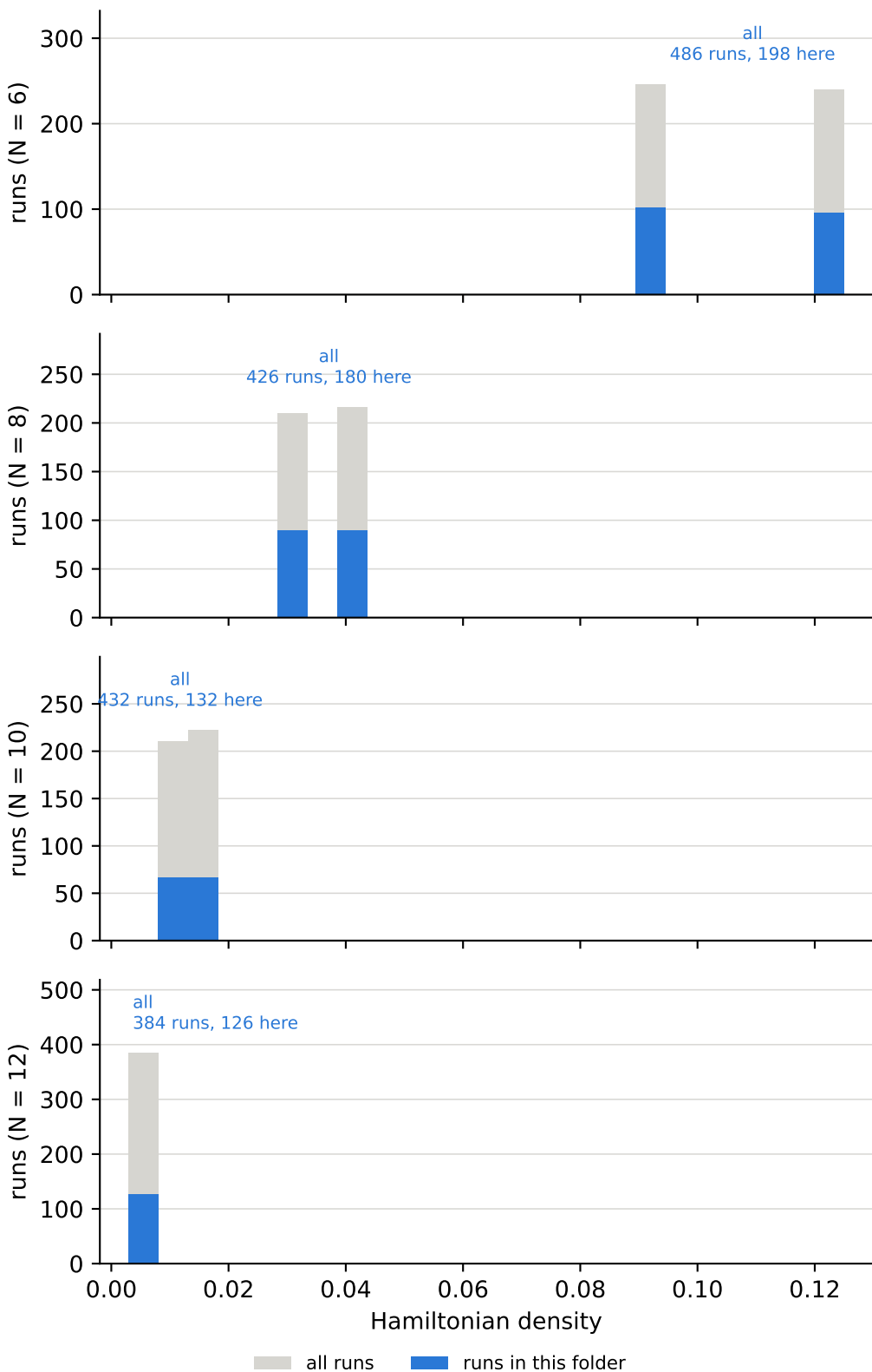
Hamiltonian density over all runs, and the cuts behind the bins coupling J = mid, Hamiltonian density = all
