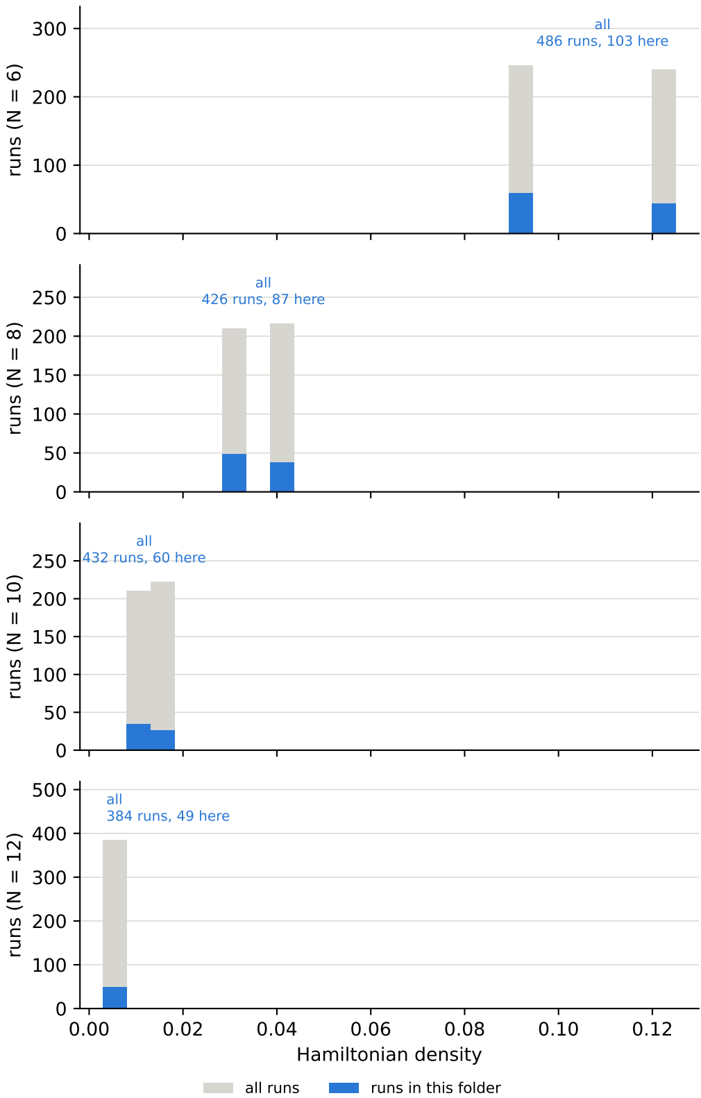
Hamiltonian density over all runs, and the cuts behind the bins coupling J = mid, Hamiltonian density = all, initial overlap = low
