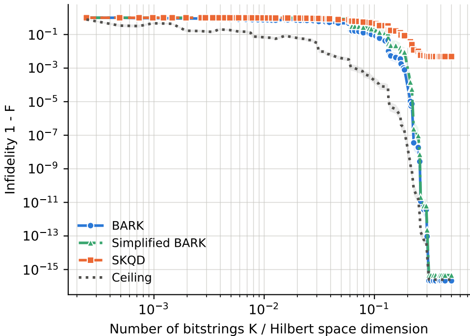
runs per point -- BARK: 53-209, Ceiling: 53-209, SKQD: 53-209, Simplified BARK: 53-209
