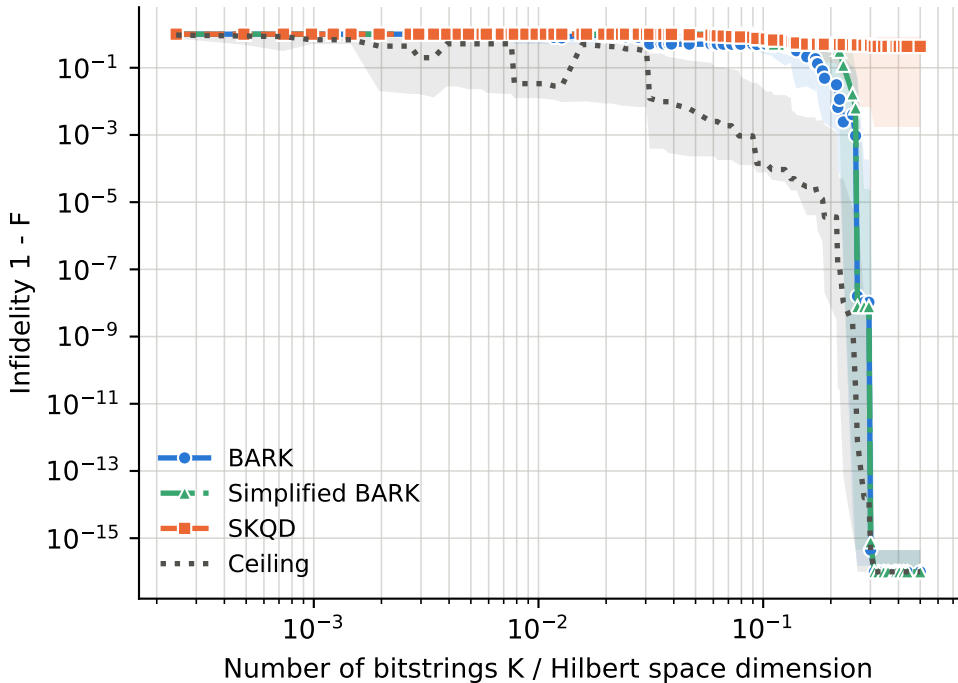
runs per point -- BARK: 49-299, Ceiling: 49-299, SKQD: 49-299, Simplified BARK: 49-299
