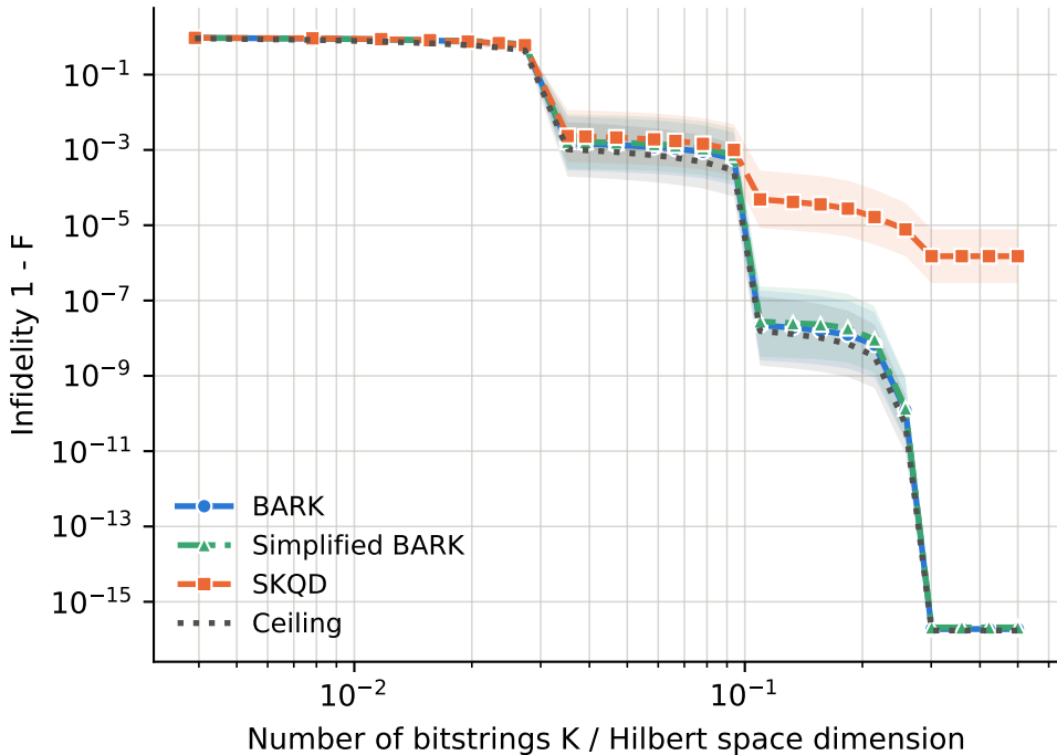
N = 8, coupling J = low, initial overlap = high (band: standard error)
