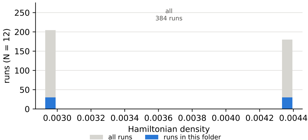
Hamiltonian density over all runs, and the cuts behind the bins N = 12 , anisotropy \delta = 1
