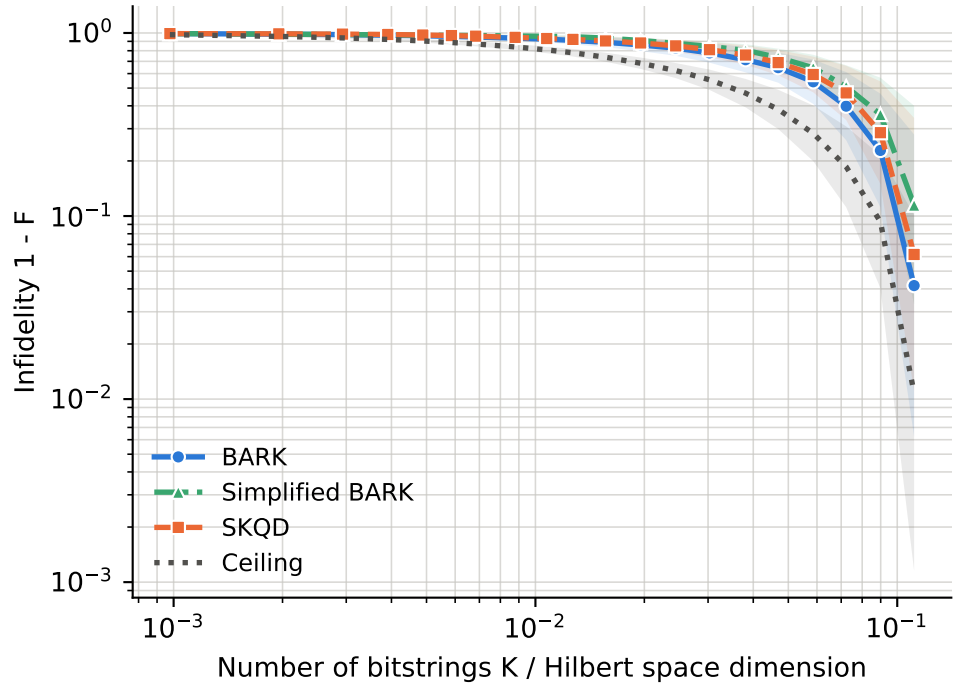
runs per point -- BARK: 60, Ceiling: 60, SKQD: 60, Simplified BARK: 60
