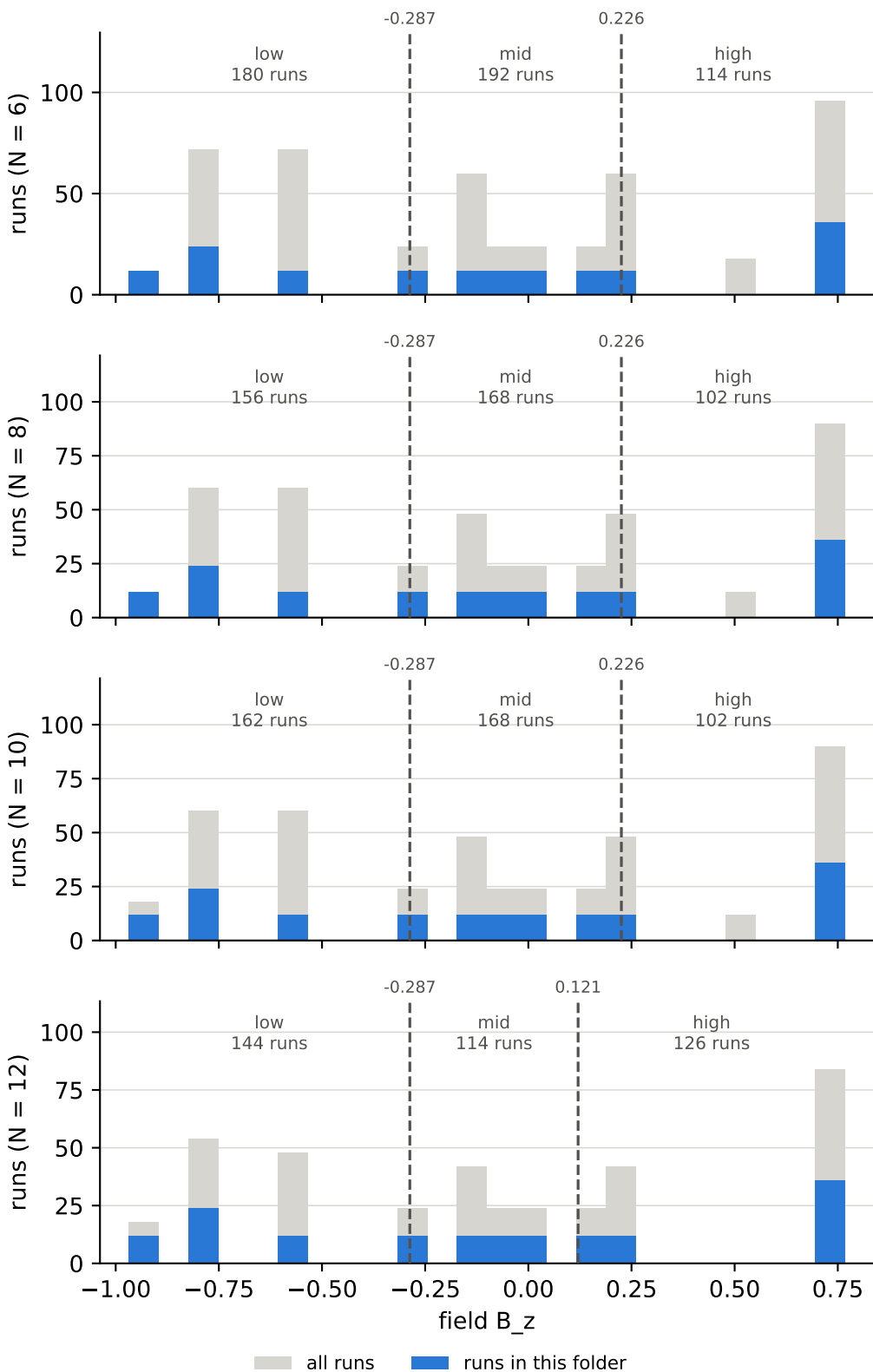
field B_z over all runs, and the cuts behind the bins anisotropy delta = 0
