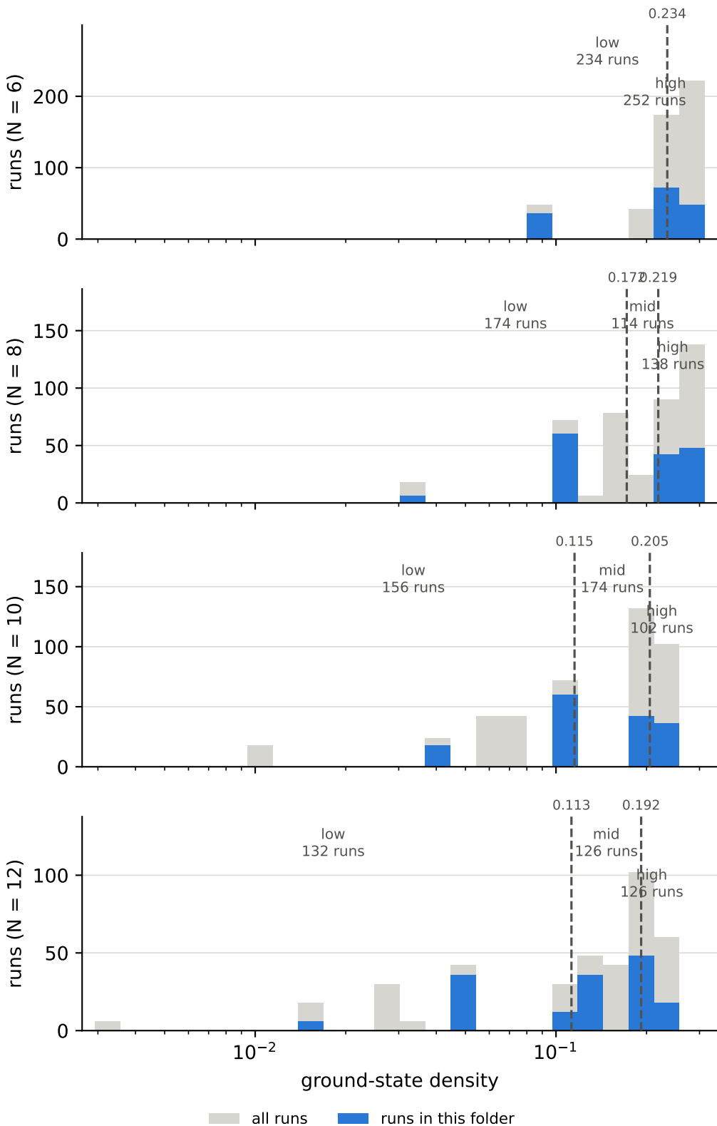
ground-state density over all runs, and the cuts behind the bins anisotropy \Delta = 0
