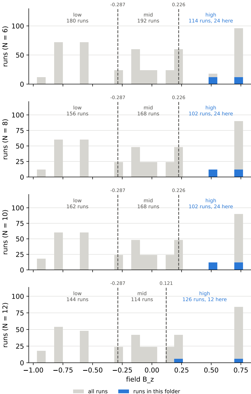
field B z over all runs, and the cuts behind the bins anisotropy delta = 10, field B z = high
