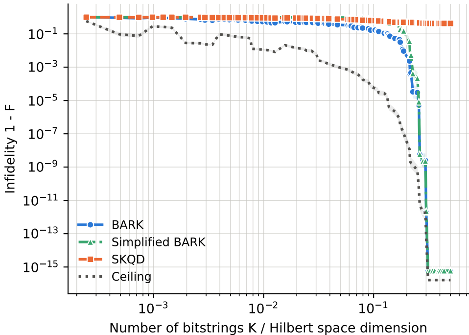
runs per point -- BARK: 18-174, Ceiling: 18-174, SKQD: 18-174, Simplified BARK: 18-174
