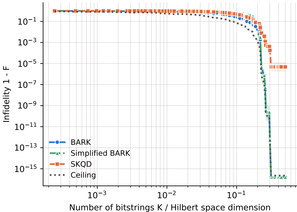
anisotropy delta = 1, coupling J = mid (band: standard error)
