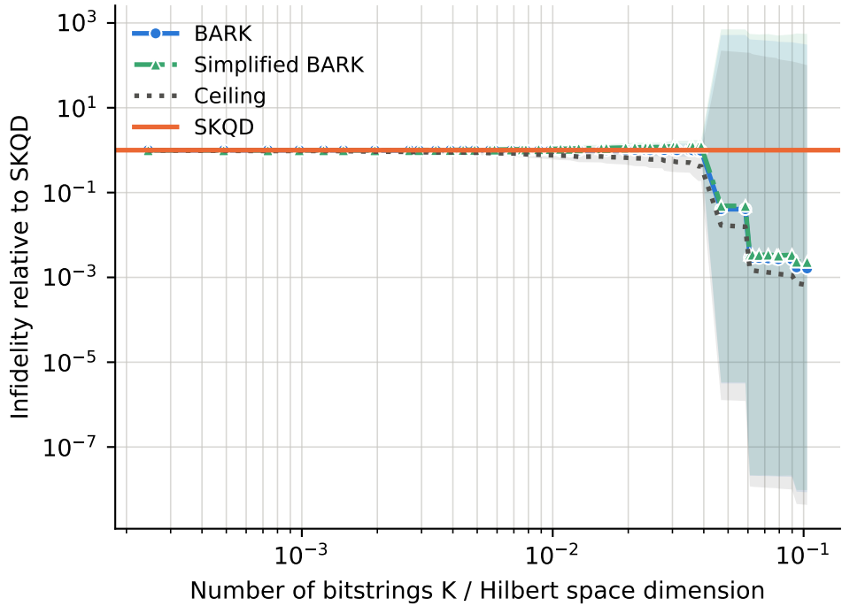
runs per point -- BARK: 19-77, Ceiling: 19-77, SKQD: 19-77, Simplified BARK: 19-77
