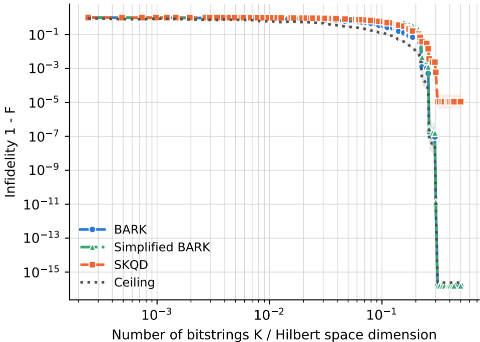
anisotropy delta = 1, ground-state density = high (band: standard error)
