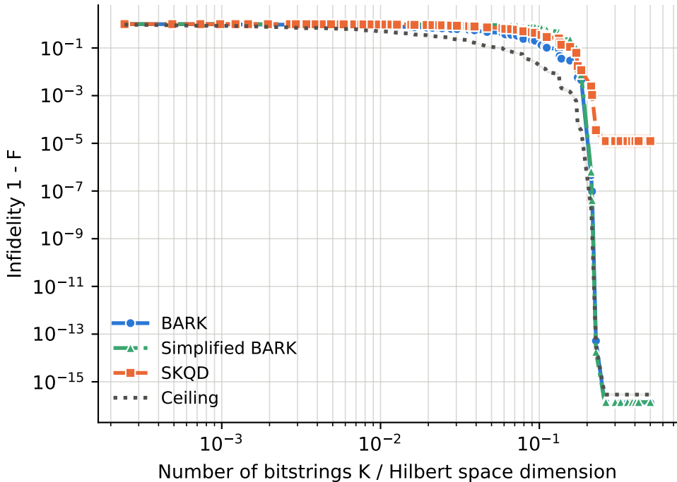
runs per point -- BARK: 48-102, Ceiling: 48-102, SKQD: 48-102, Simplified BARK: 48-102
