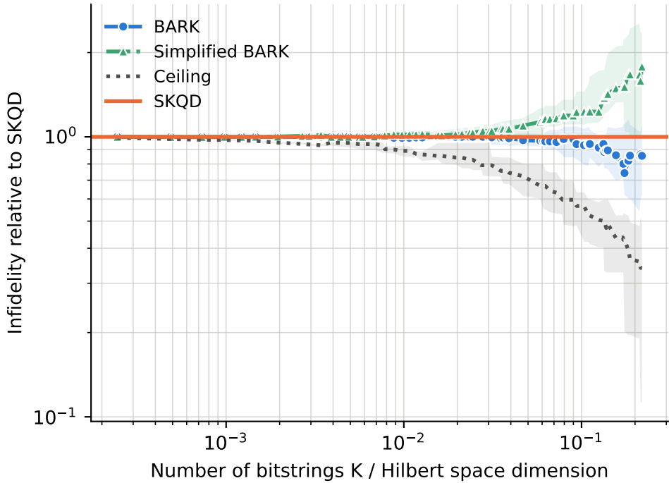
runs per point -- BARK: 12-55, Ceiling: 12-55, SKQD: 12-55, Simplified BARK: 12-55
