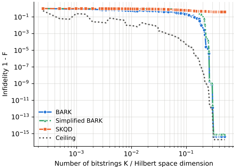
anisotropy delta = 10, Hamiltonian density = all (band: standard error)
