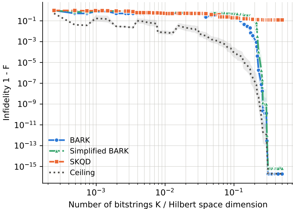
anisotropy delta = 10, initial overlap = high (band: standard error)
