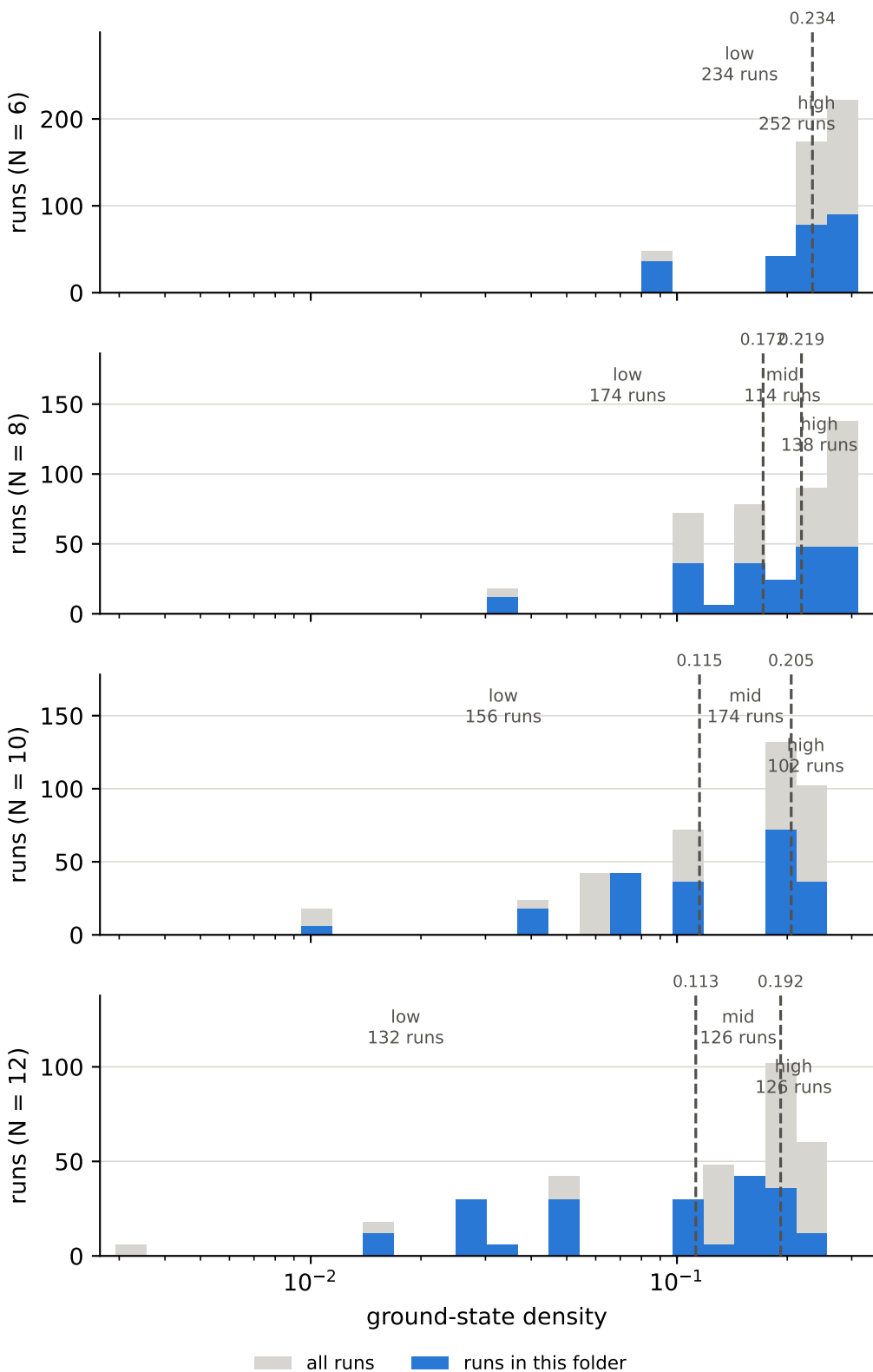
ground-state density over all runs, and the cuts behind the bins lattice dimension = 1
