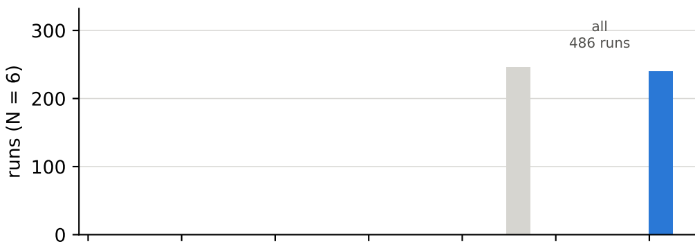
Hamiltonian density over all runs, and the cuts behind the bins lattice dimension = 2
