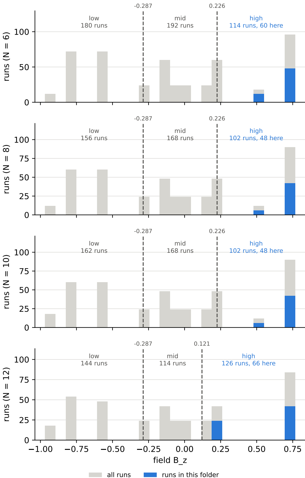
field B z over all runs, and the cuts behind the bins lattice dimension = 1, field B z = high
