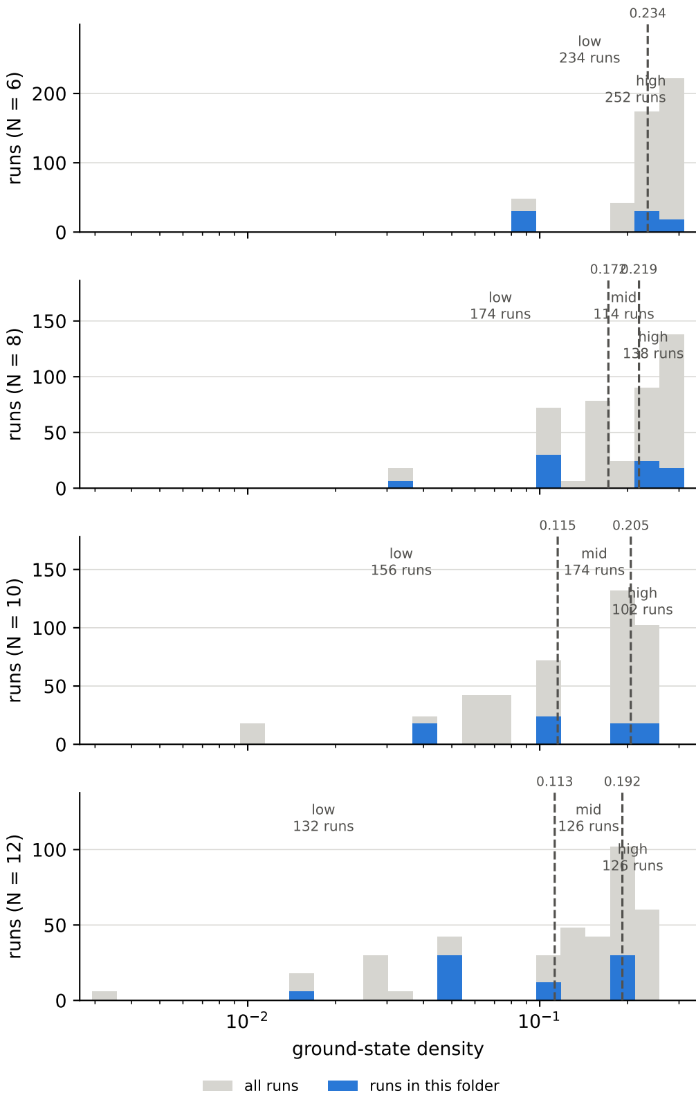
ground-state density over all runs, and the cuts behind the bins lattice dimension = 1, anisotropy \delta = 0
