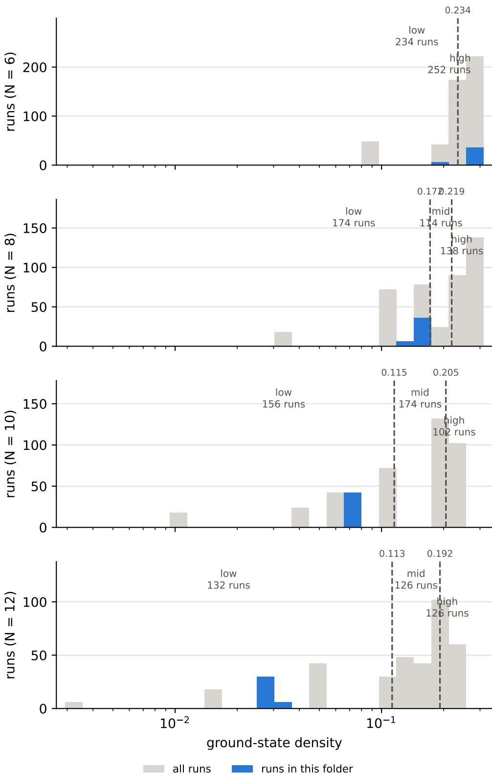
ground-state density over all runs, and the cuts behind the bins lattice dimension = 1, anisotropy delta = 10
