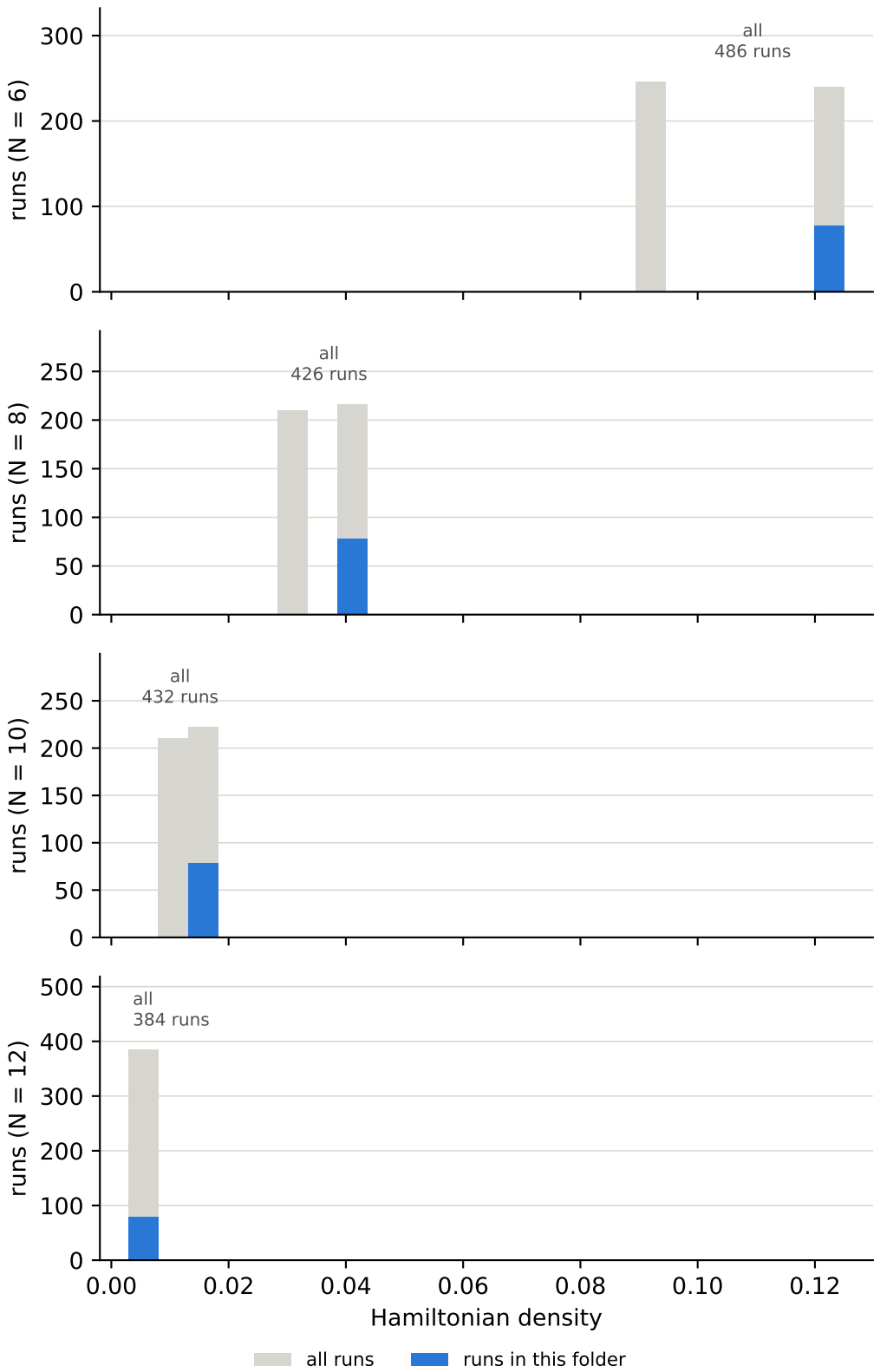
Hamiltonian density over all runs, and the cuts behind the bins lattice dimension = 2, anisotropy delta = 0
