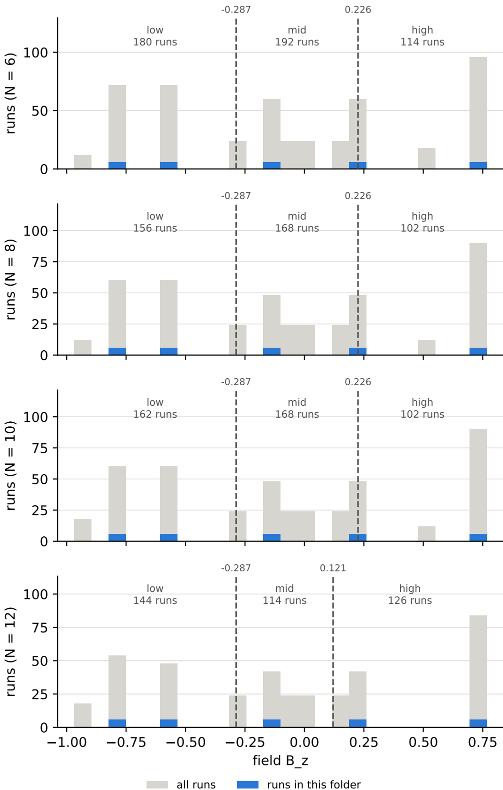
field B_z over all runs, and the cuts behind the bins lattice dimension = 2, anisotropy \delta = 1
