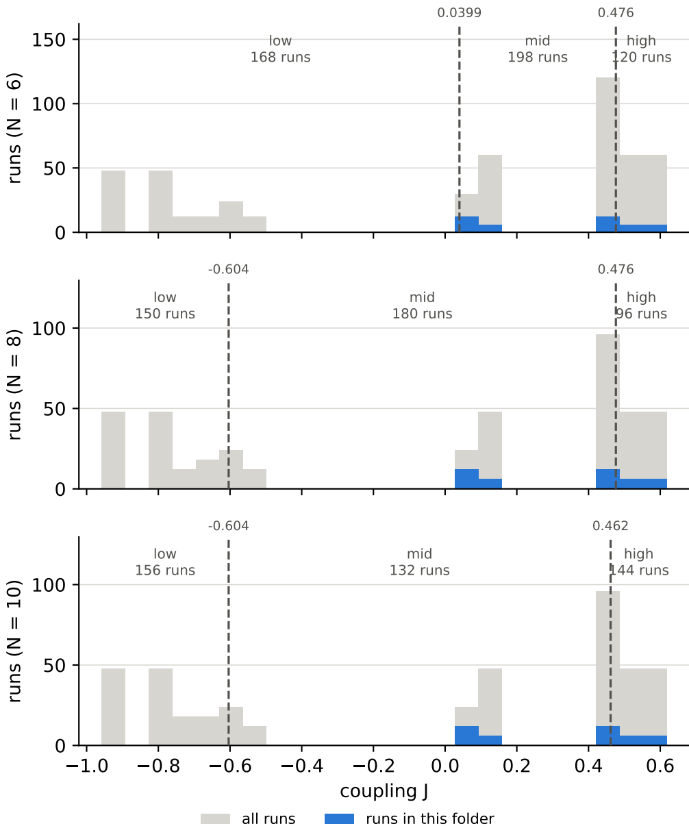
coupling J over all runs, and the cuts behind the bins lattice dimension = 2, anisotropy \Delta = 10
