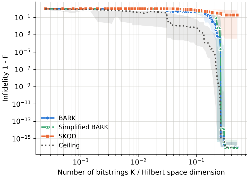
runs per point -- BARK: 128-580, Ceiling: 128-580, SKQD: 128-580, Simplified BARK: 128-580
