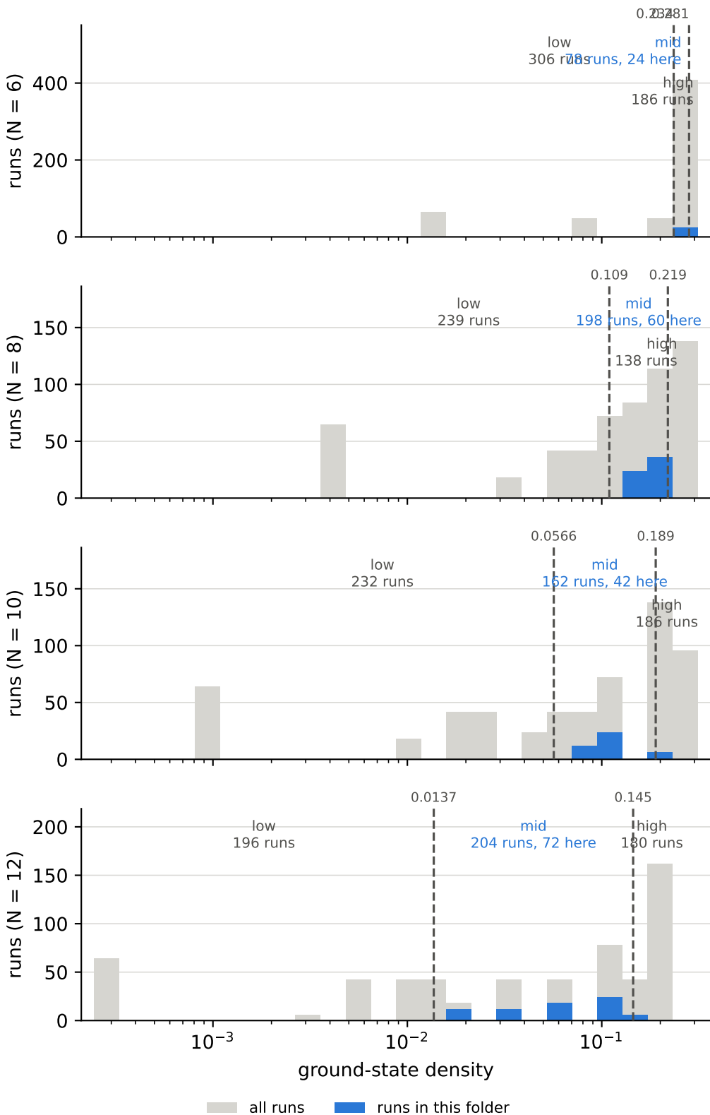
ground-state density over all runs, and the cuts behind the bins field B_z = high, ground-state density = mid
