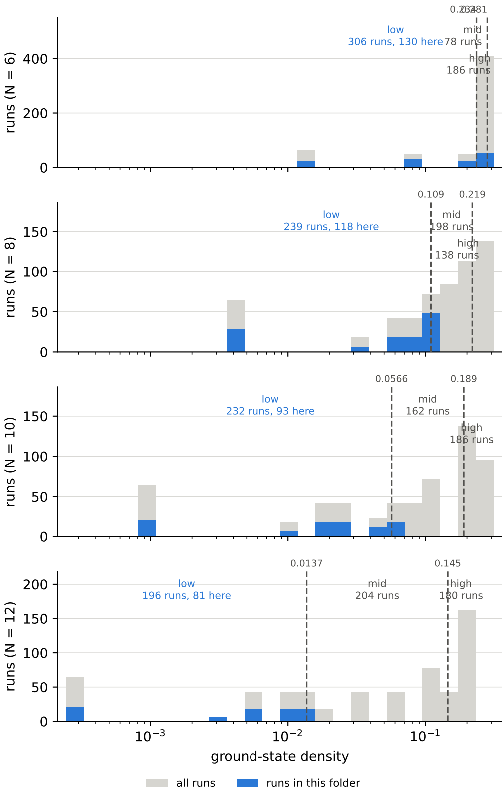
ground-state density over all runs, and the cuts behind the bins field B_z = low, ground-state density = low
