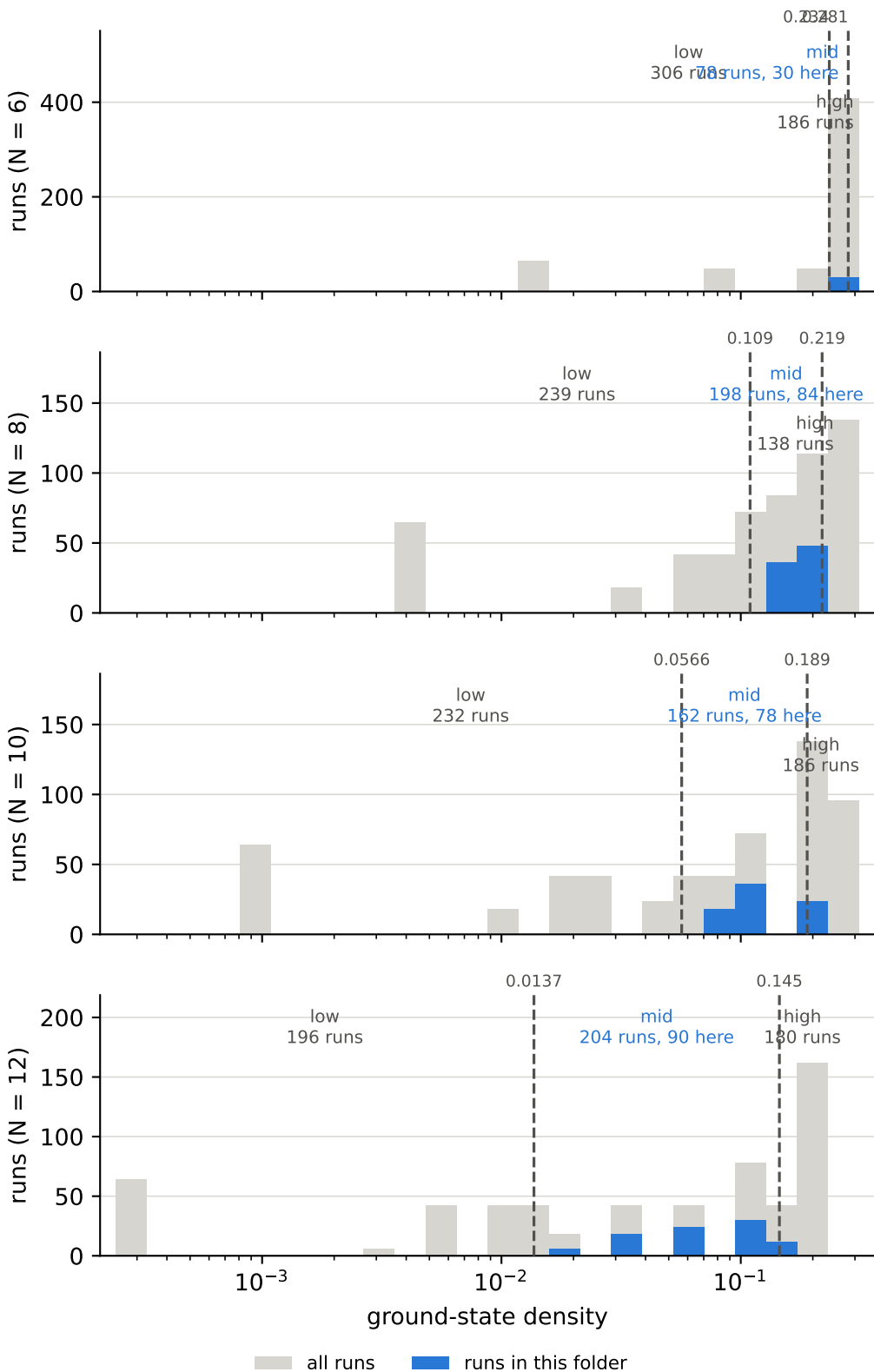
ground-state density over all runs, and the cuts behind the bins field B_z = low, ground-state density = mid
