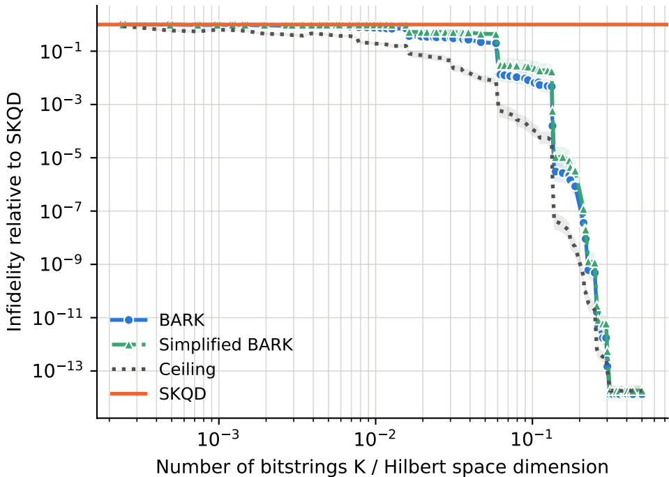
runs per point -- BARK: 90-282, Ceiling: 90-282, SKQD: 90-282, Simplified BARK: 90-282
