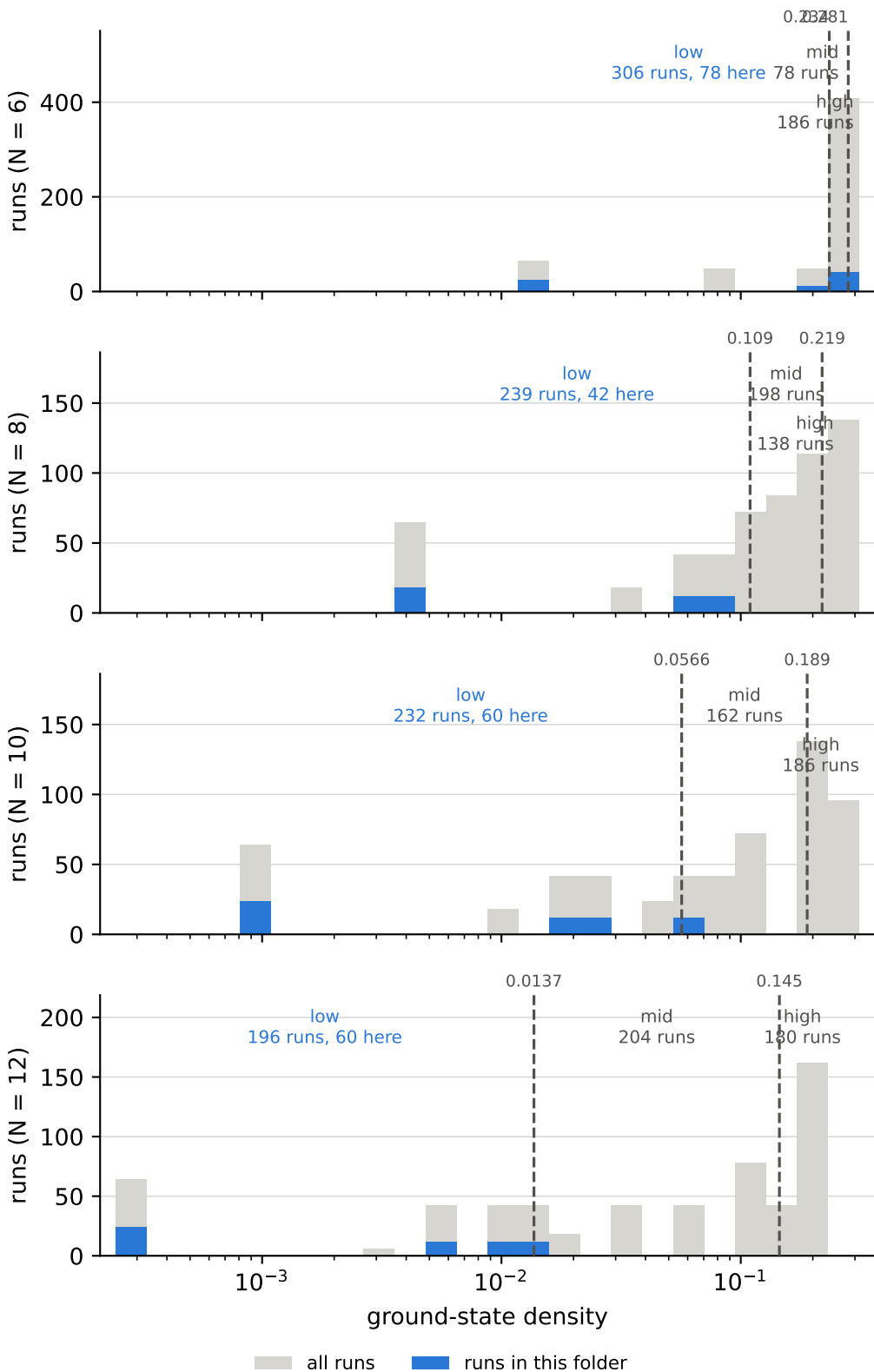
ground-state density over all runs, and the cuts behind the bins field B_z = mid, ground-state density = low
